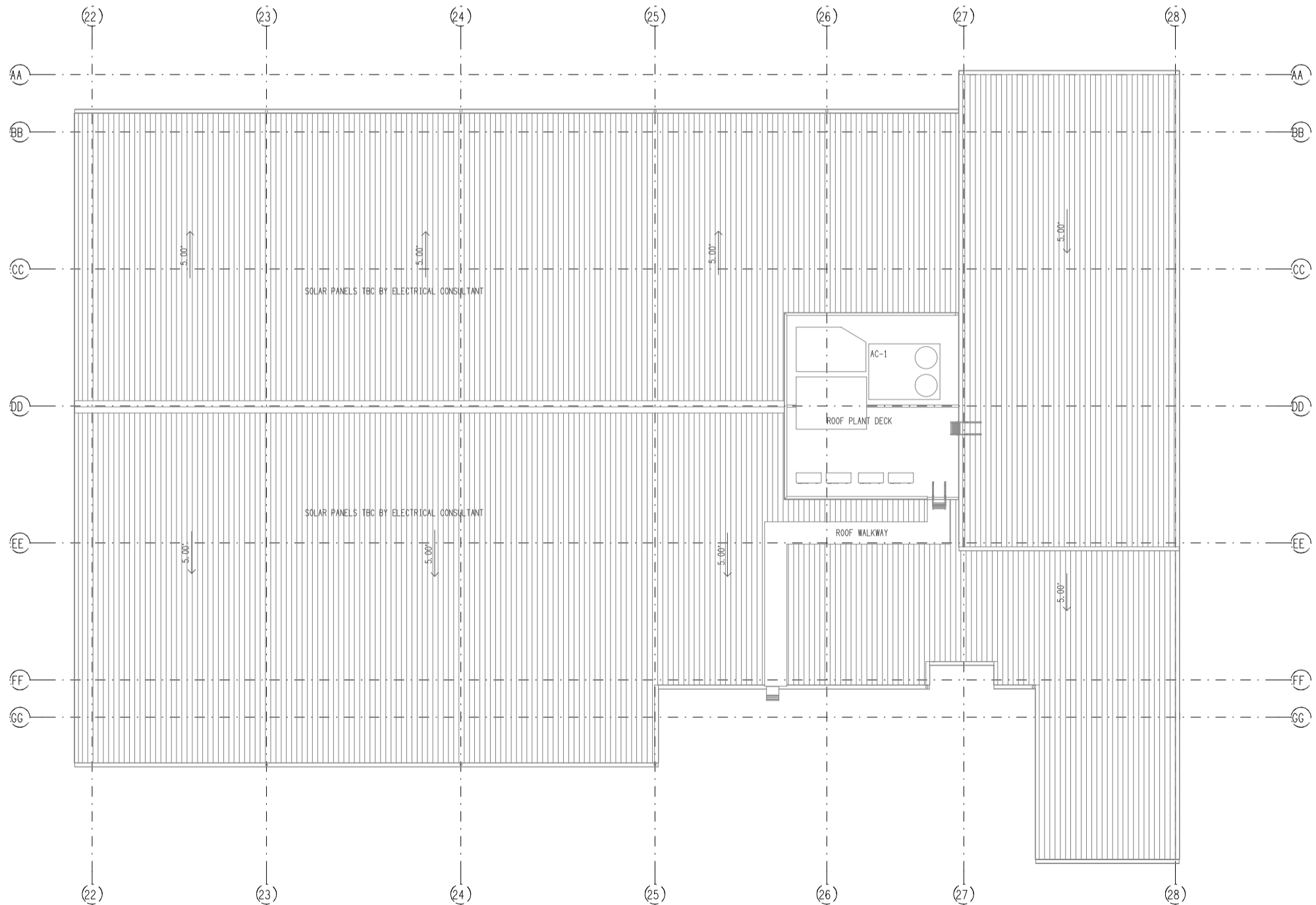
BOTTLE SHOP ROOF PLAN PLANT DECK LAYOUT SCALE 1:200
